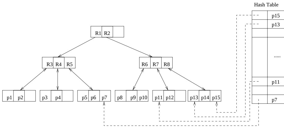
Fig. 2. Secondary Index Access to R-Tree Leaves
