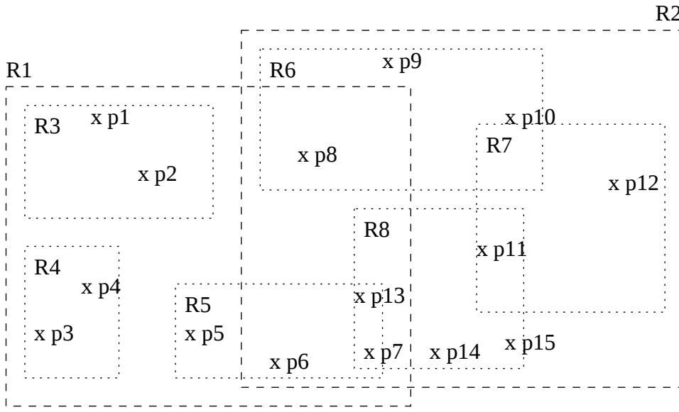
(a) Planar representation of R-tree
