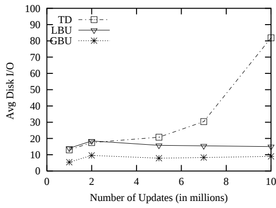
(a) Varying Amounts of Updates, Update
