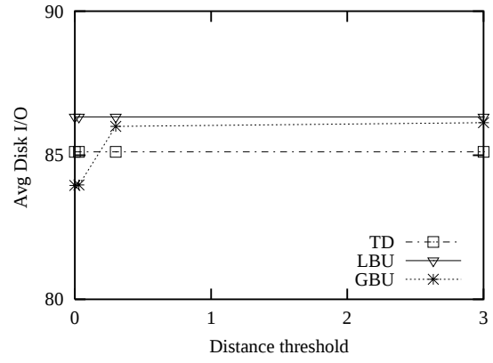
(b) Varying \theta , Querying
