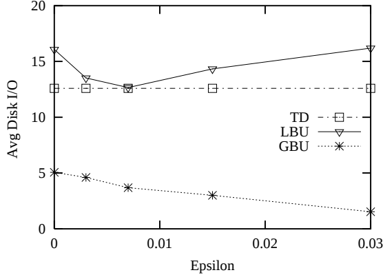
(a) Varying \epsilon : Average Disk I/O, Update
