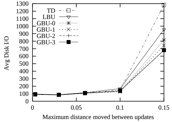
(b) Ascending the R-Tree, Querying
