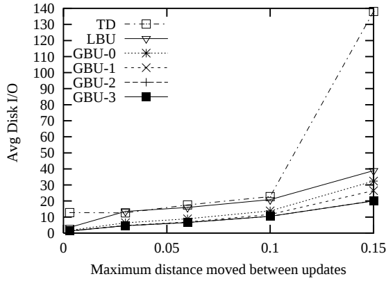
(a) Ascending the R-Tree, Update
