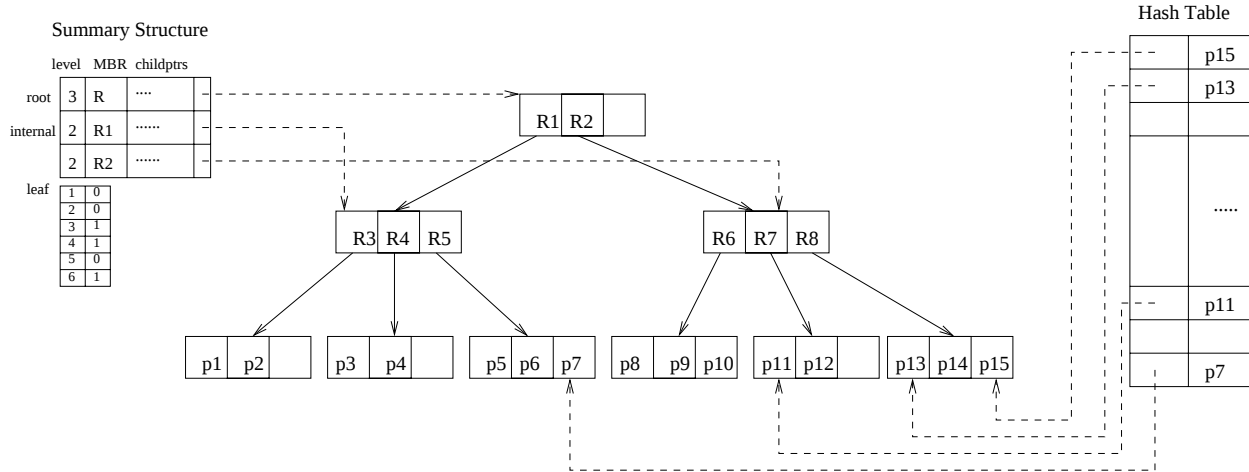
Fig. 3. Summary Structure for an R-Tree
