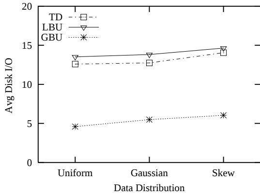
(c) Varying Data Distributions, Update
