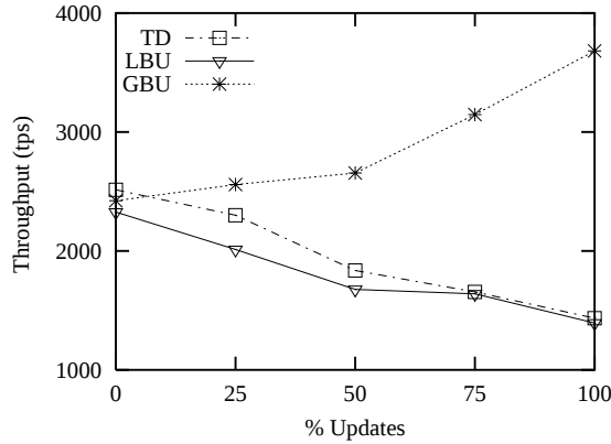
Fig. 11. Throughput for Varying Mix of Updates and Window Queries
