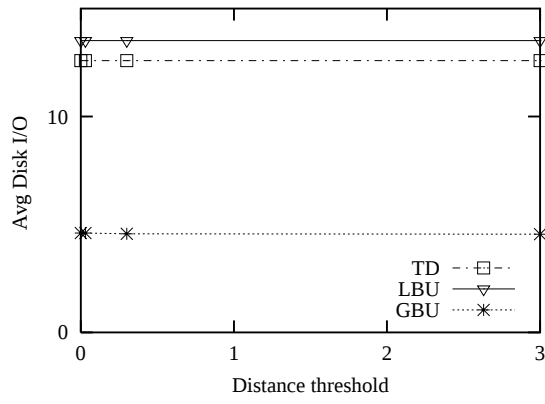
(a) Varying \theta , Update
