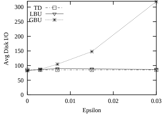
(b) Varying \epsilon : Average Disk I/O, Querying
