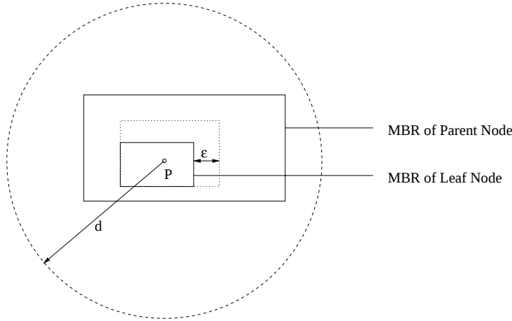
Fig. 5. The movement of point for cost analysis
