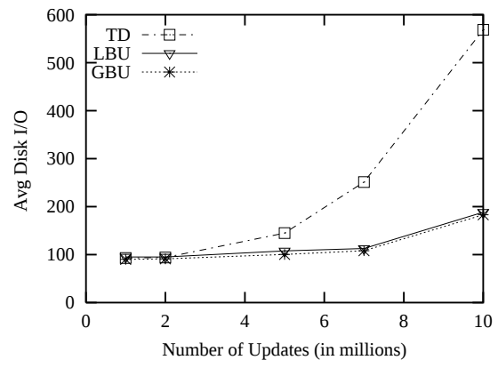
(b) Varying Amounts of Updates, Querying
