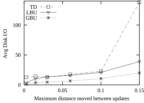
(c) Varying Maximum Distance, Update
