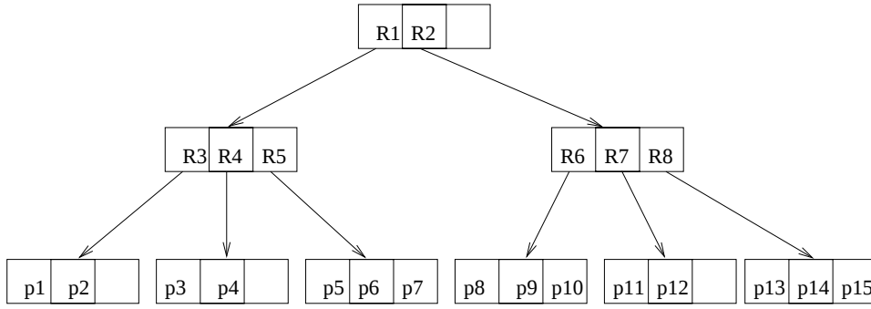
(b) Directory of R-tree
