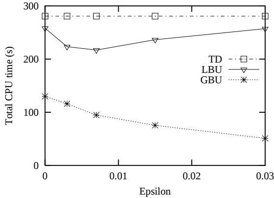
(c) Varying \epsilon : Total CPU Cost, Update
