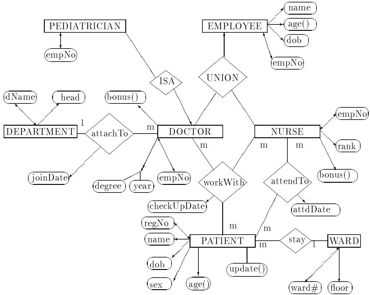
Fig 3. Normal Form OER Diagram
