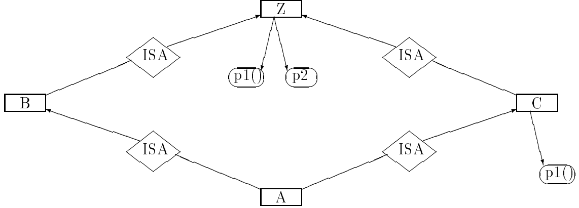
Fig 2. An Inheritance Diagram
